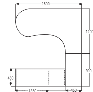
CS-118 Top 25mm Thick PLPB / MDF or Postformed Legs 18/25mm Thick PLPB / MDF Storage/Pedestal 18mm Thick PLPB / MDF Modesty 18mm Thick PLPB / MDF
